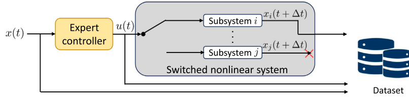
Fig. 2. Data collection phase.
